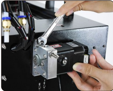
Fixed feeder
