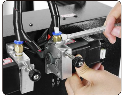
Connect joint
