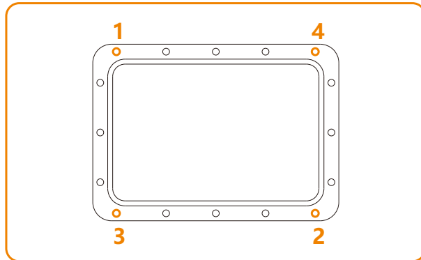
12. Follow the right sequence to install the screws at four corners according to the illustration.
