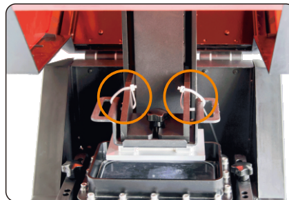
15. Cut the white tie that holds the z-axis.
