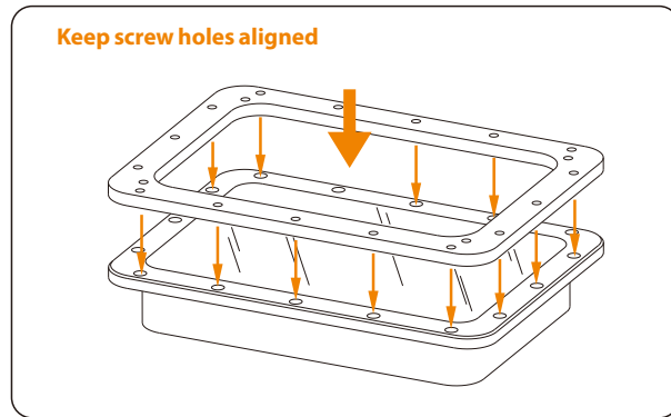
10. Put the film onto the resin vat.
